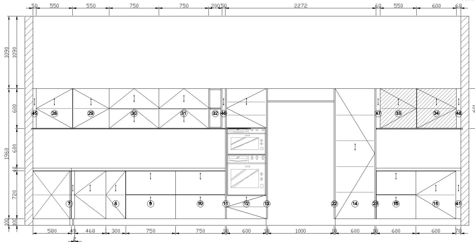
A View elevation drawing
