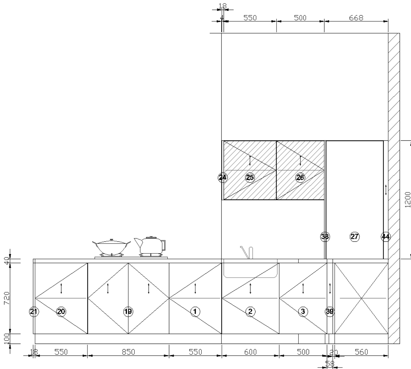
C View elevation drawing
