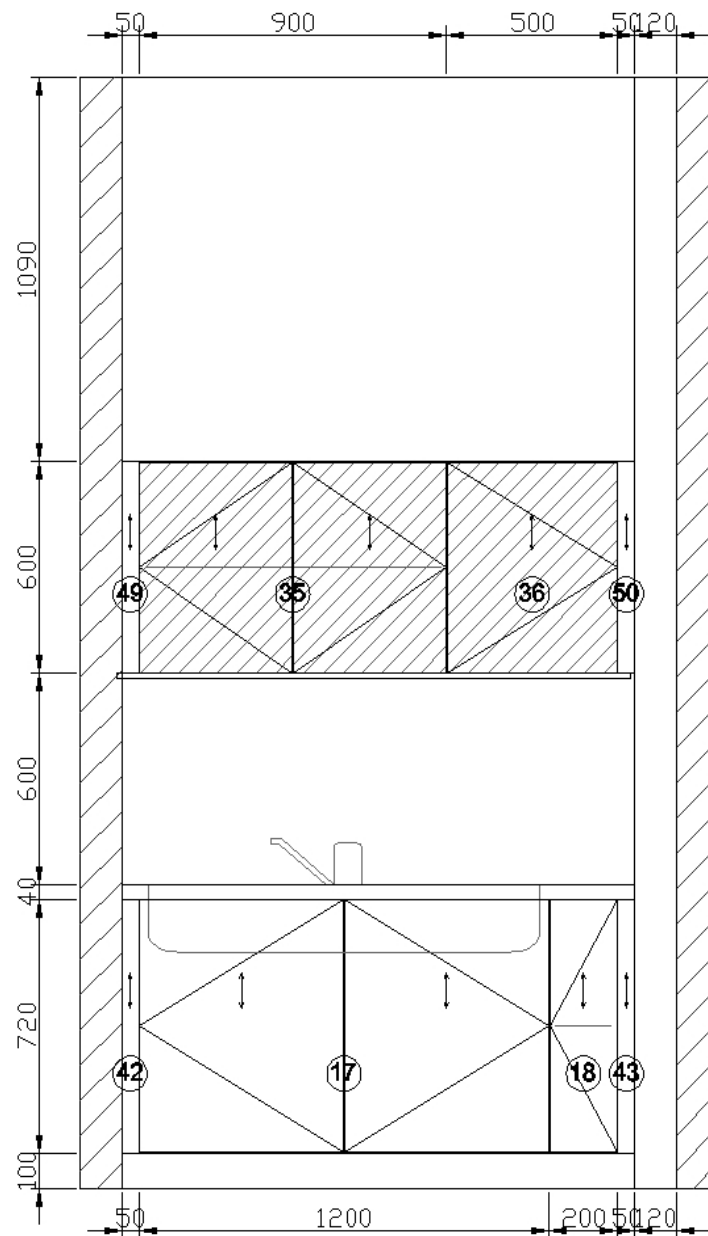
B View elevation drawing
